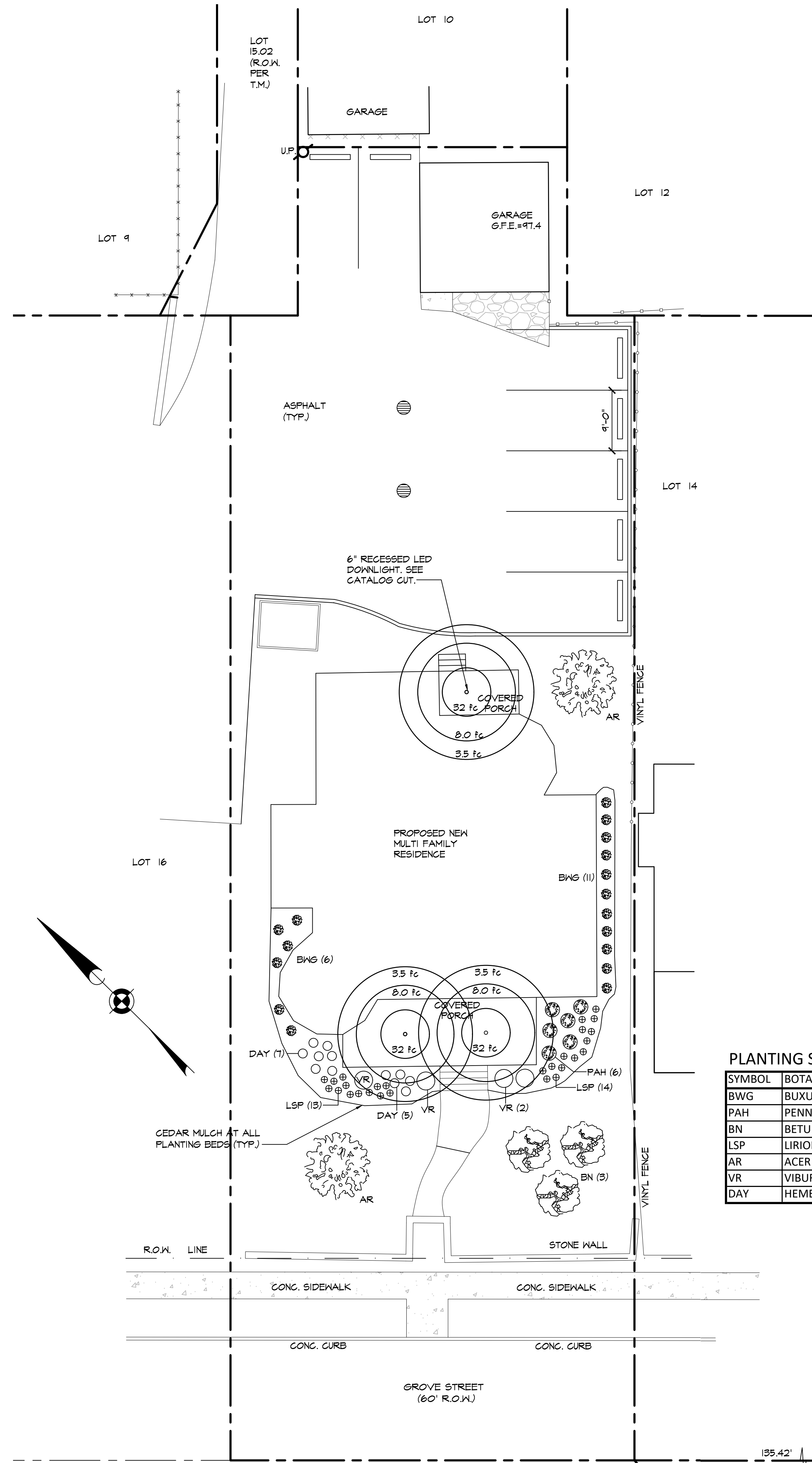
LANDSCAPING AND LIGHTING PLAN SCALE: 1" = 10'-0"
